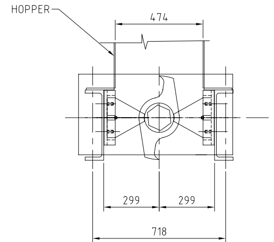
VIEW (B) SCALE 1:5 SHOWS CUTTERS AND FINGERS
